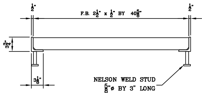
FRAME ELEVATION VIEW
