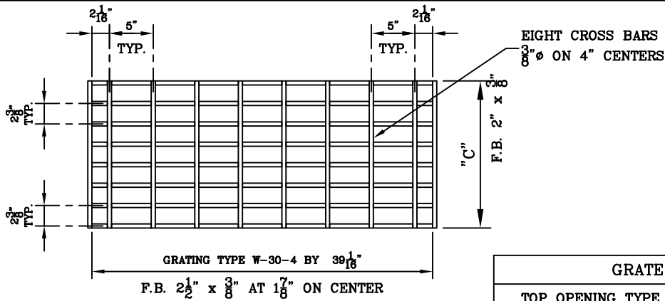
BAR GRATE PLAN VIEW
