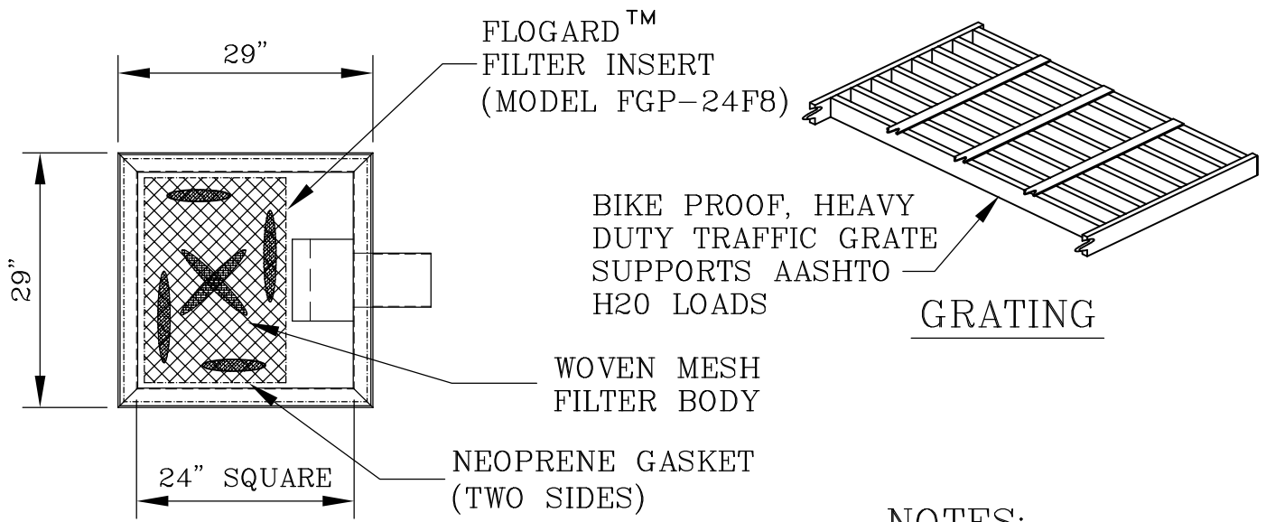
PLAN VIEW
