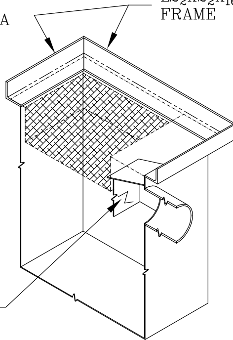
ISOMETRIC SECTION
