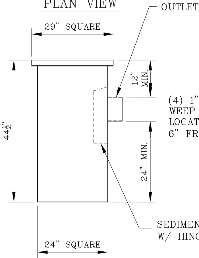
SIDE VIEW
