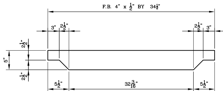
MIDDLE BAR OF GRATE
