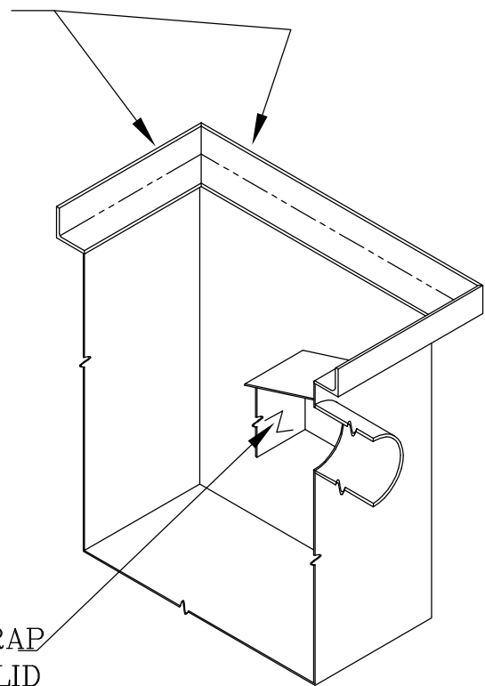
ISOMETRIC SECTION
